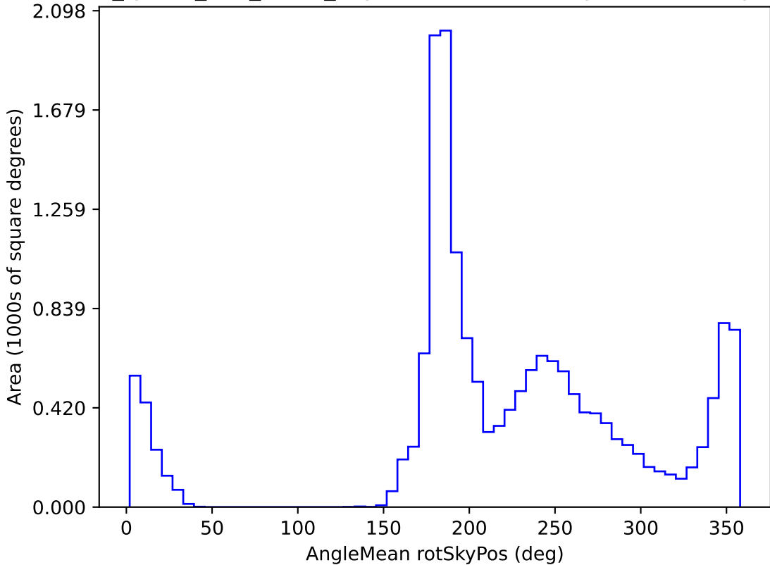
too_ignore_100_1v3.4_10yrs WFD i band: AngleMean rotSkyPos
