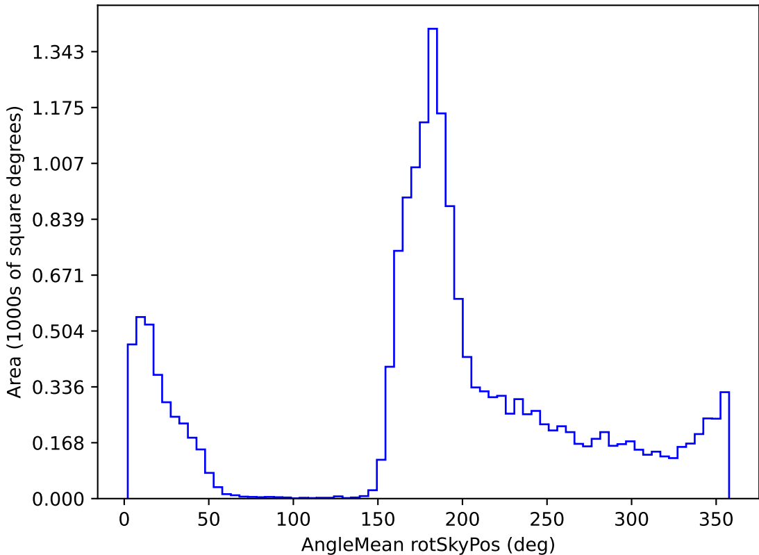
too_ignore_100_1v3.4_10yrs WFD g band: AngleMean rotSkyPos
