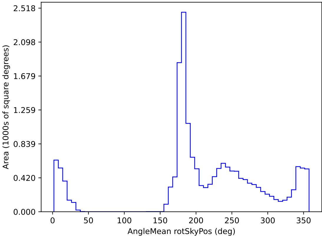
too_ignore_100_1v3.4_10yrs WFD all bands: AngleMean rotSkyPos
