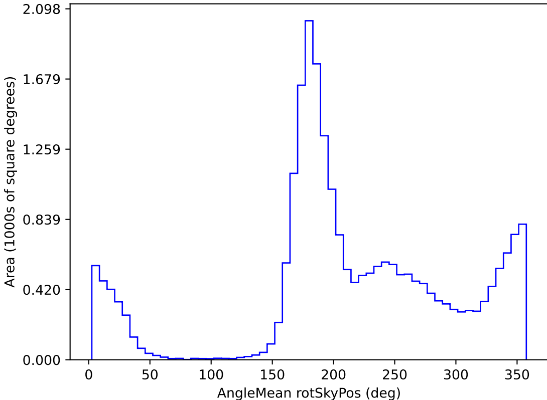
too_ignore_100_1v3.4_10yrs All sky u band: AngleMean rotSkyPos
