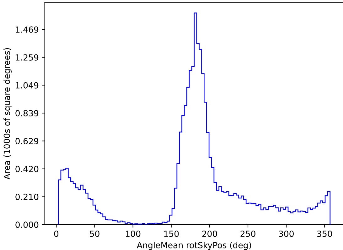
too_ignore_100_1v3.4_10yrs All sky g band: AngleMean rotSkyPos
