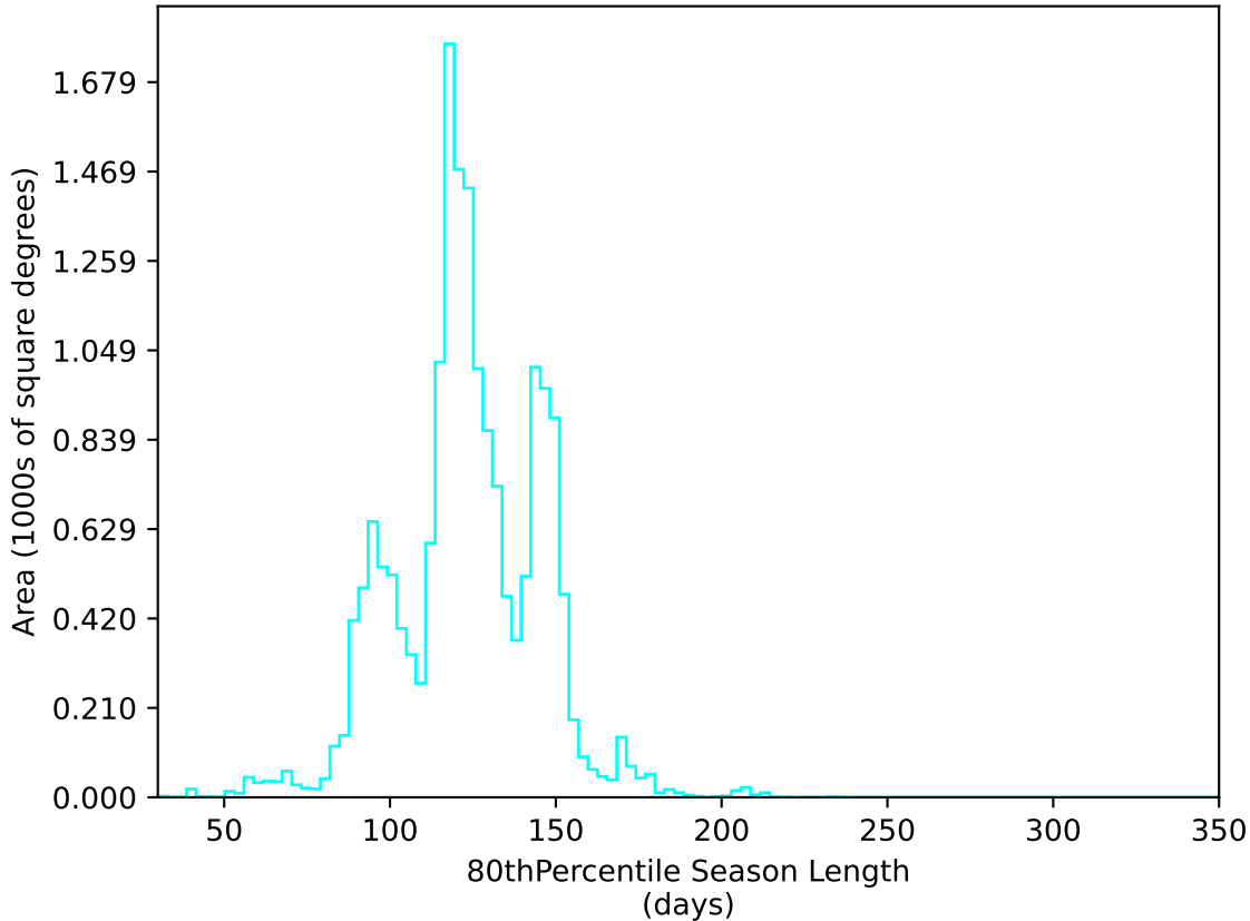
too_ignore_100_1v3.4_10yrs WFD u band: 80thPercentile Season Length
