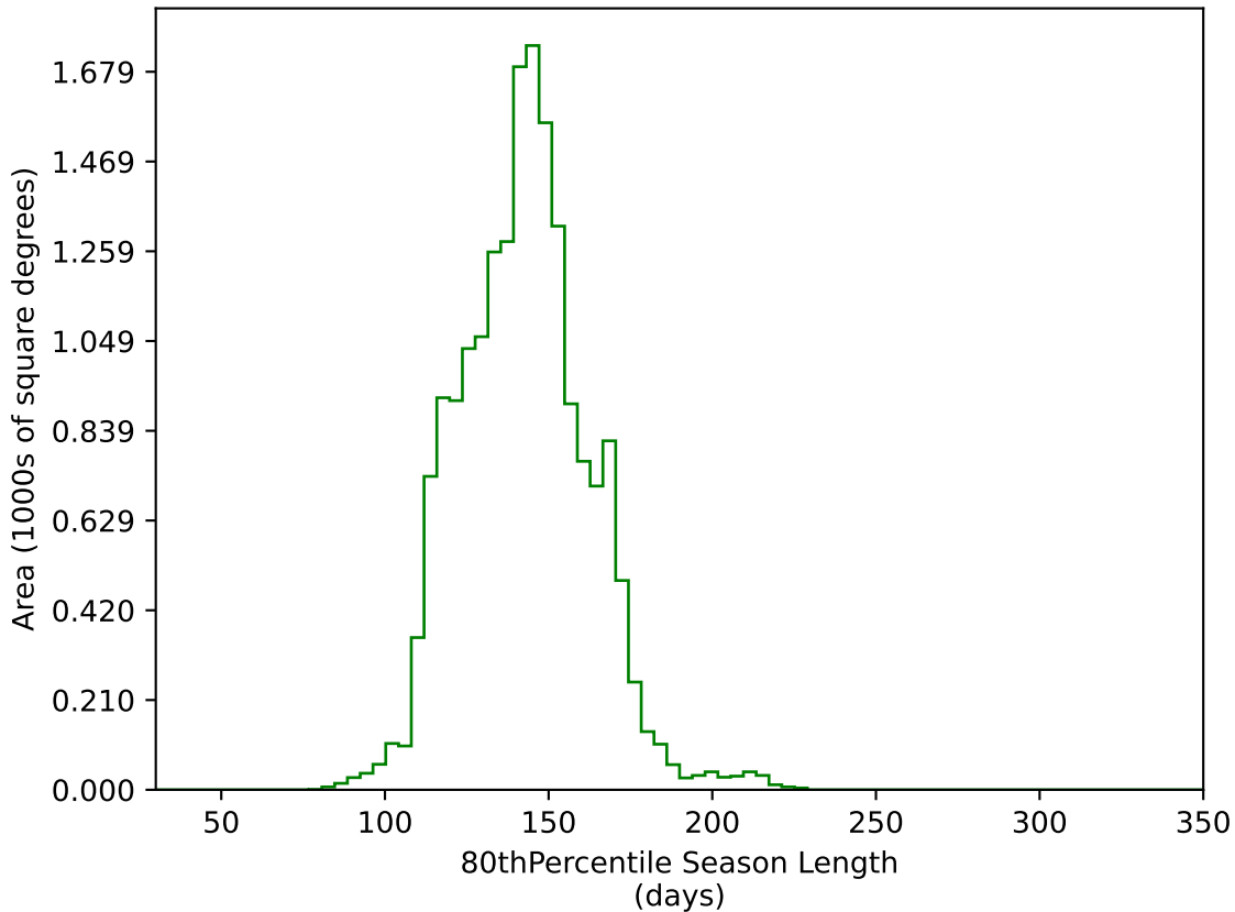
too_ignore_100_1v3.4_10yrs WFD g band: 80thPercentile Season Length
