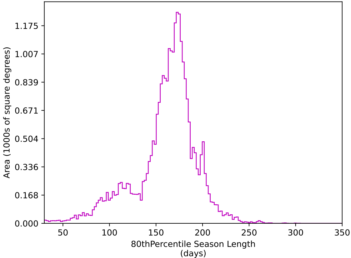
too_ignore_100_1v3.4_10yrs All sky z band: 80thPercentile Season Length
