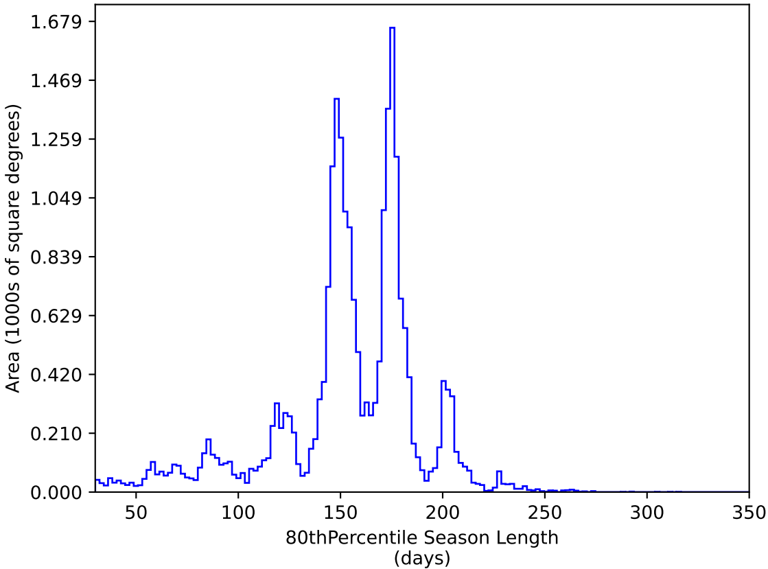
too_ignore_100_1v3.4_10yrs All sky y band: 80thPercentile Season Length
