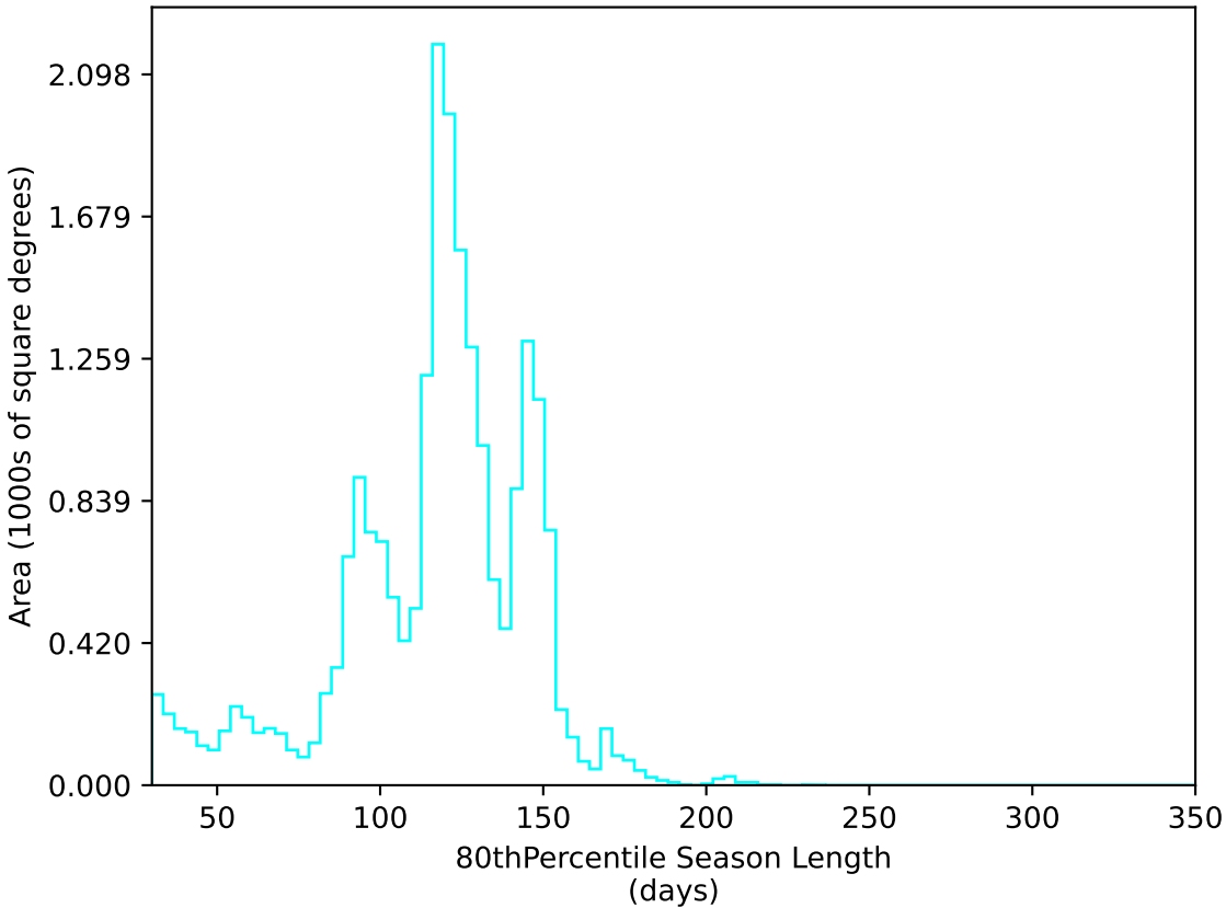
too_ignore_100_1v3.4_10yrs All sky u band: 80thPercentile Season Length
