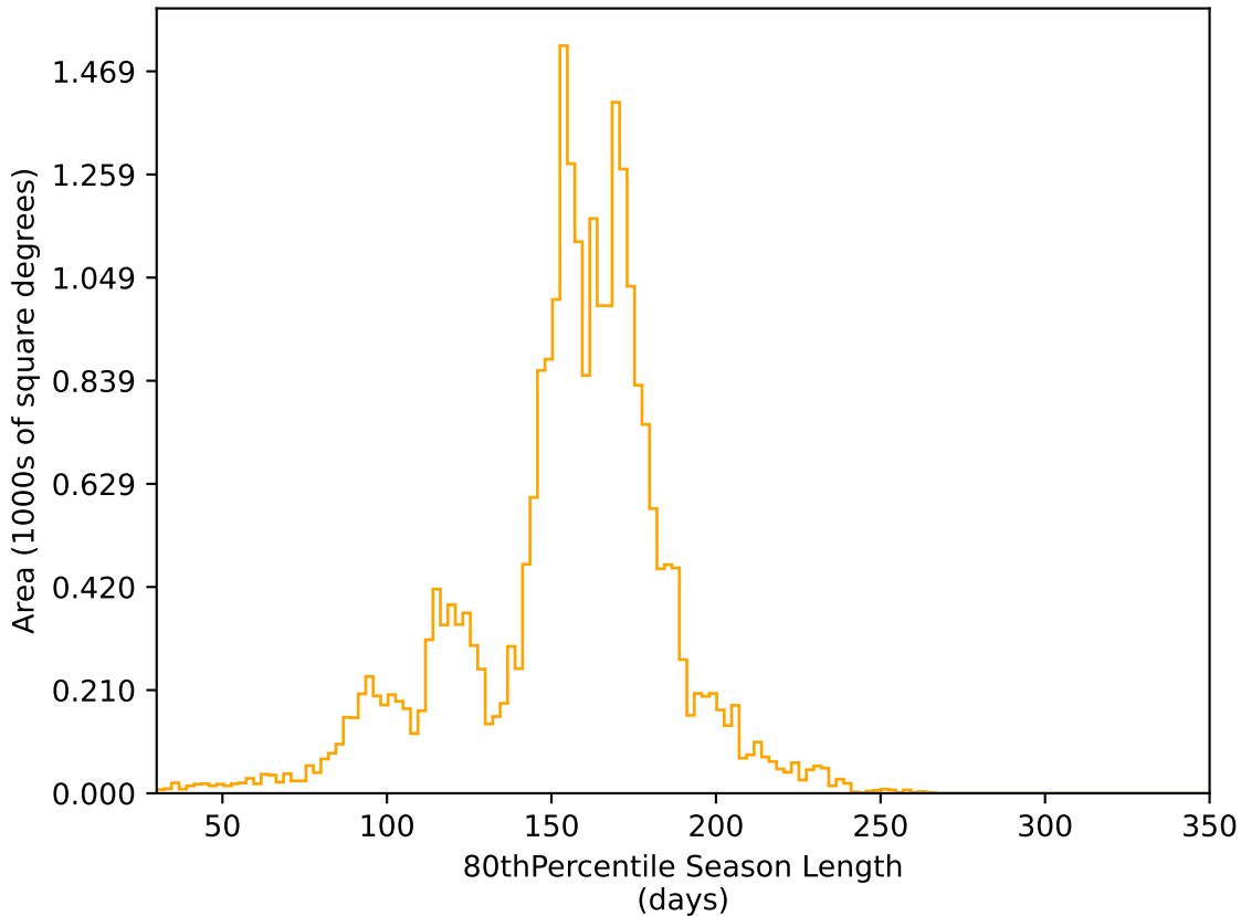
too_ignore_100_1v3.4_10yrs All sky r band: 80thPercentile Season Length
