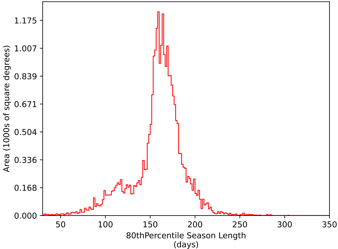
too_ignore_100_1v3.4_10yrs All sky i band: 80thPercentile Season Length
