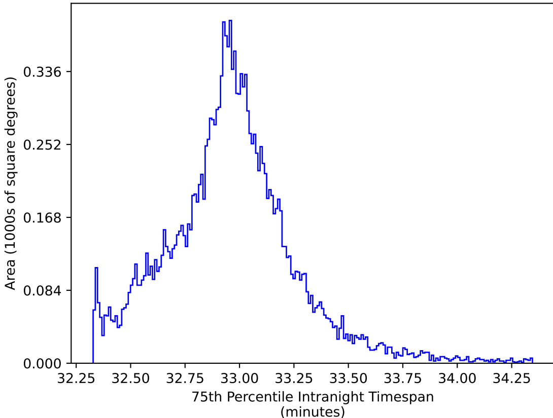
too_ignore_100_1v3.4_10yrs WFD y band: 75th Percentile Intranight Timespan
