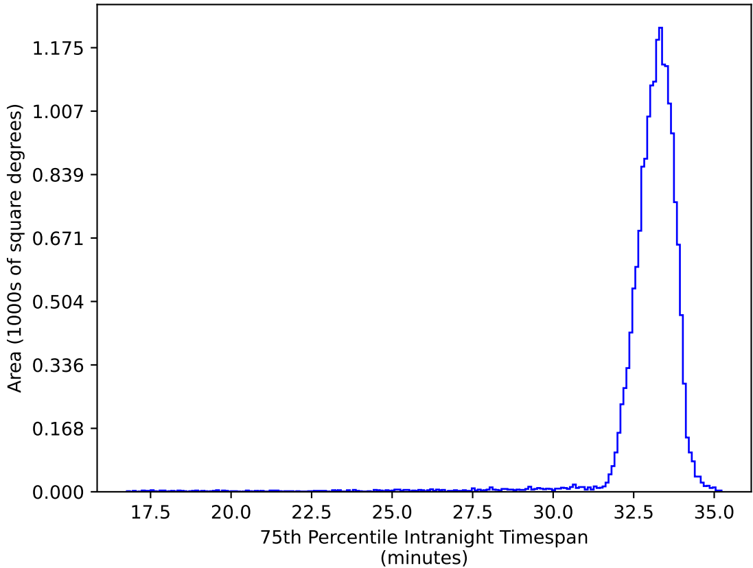
too_ignore_100_1v3.4_10yrs WFD ug bands: 75th Percentile Intranight Timespan
