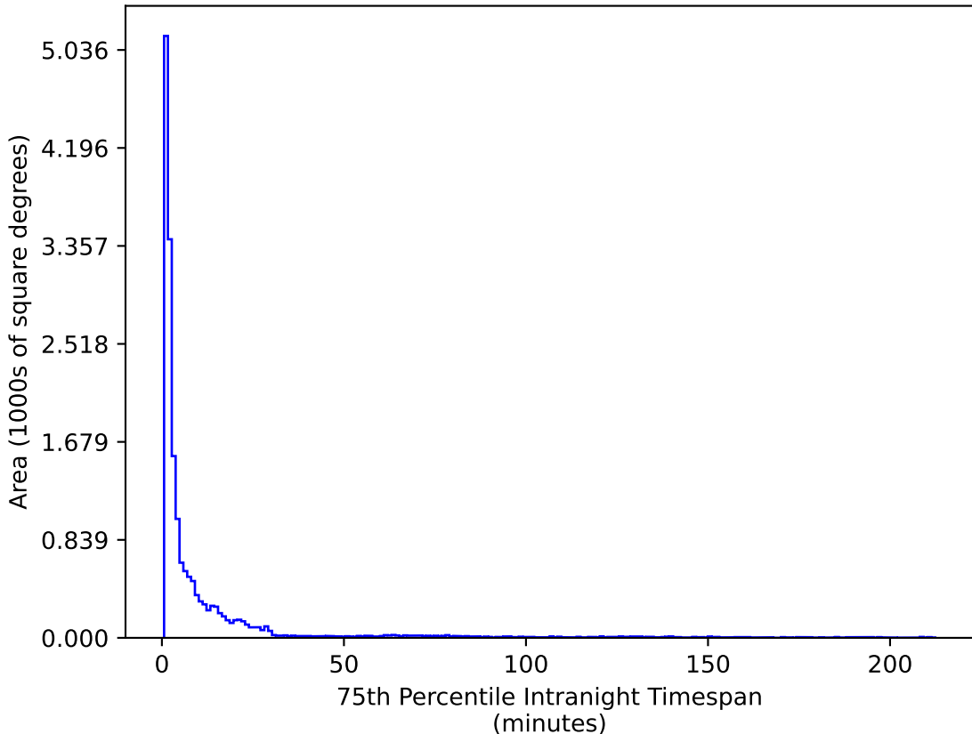
too_ignore_100_1v3.4_10yrs WFD u band: 75th Percentile Intranight Timespan
