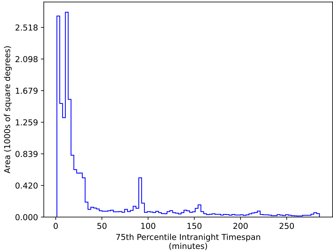
too_ignore_100_1v3.4_10yrs WFD r band: 75th Percentile Intranight Timespan
