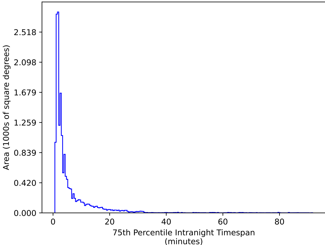
too_ignore_100_1v3.4_10yrs WFD g band: 75th Percentile Intranight Timespan
