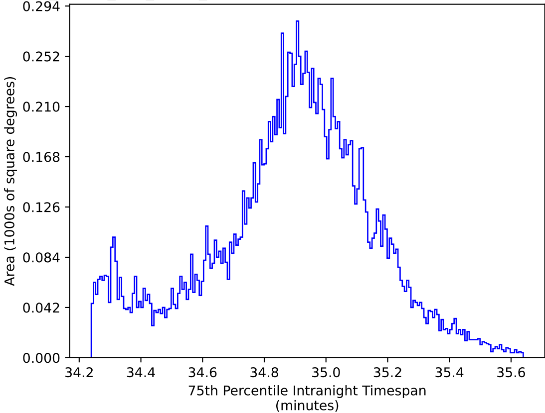
too_ignore_100_1v3.4_10yrs WFD: 75th Percentile Intranight Timespan
