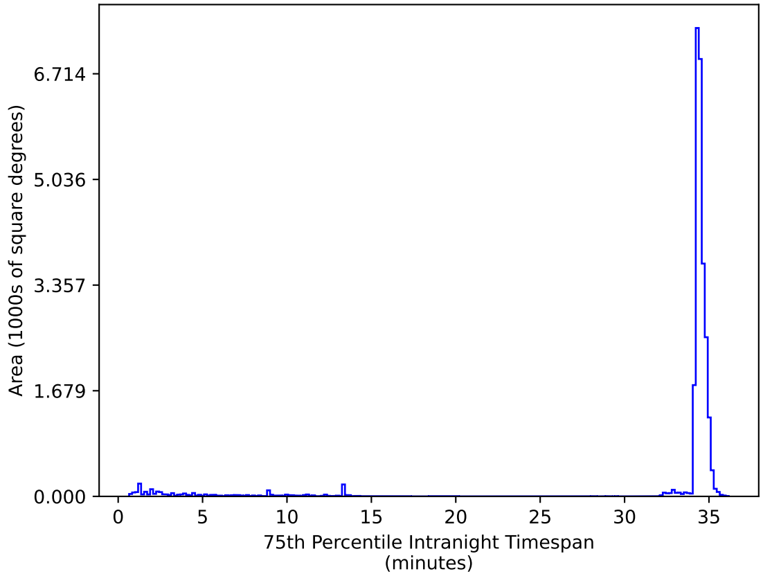
too_ignore_100_1v3.4_10yrs All sky zy bands: 75th Percentile Intranight Timespan
