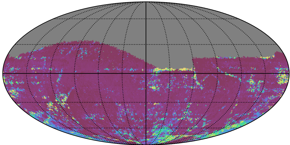
too_ignore_100_1v3.4_10yrs All sky z band: 75th Percentile Intranight Timespan
