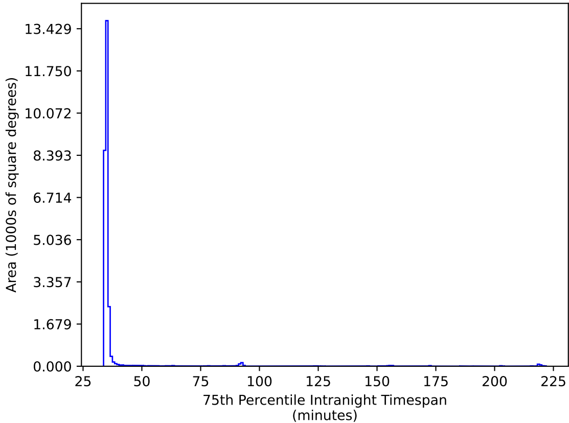
too_ignore_100_1v3.4_10yrs All sky ri bands: 75th Percentile Intranight Timespan
