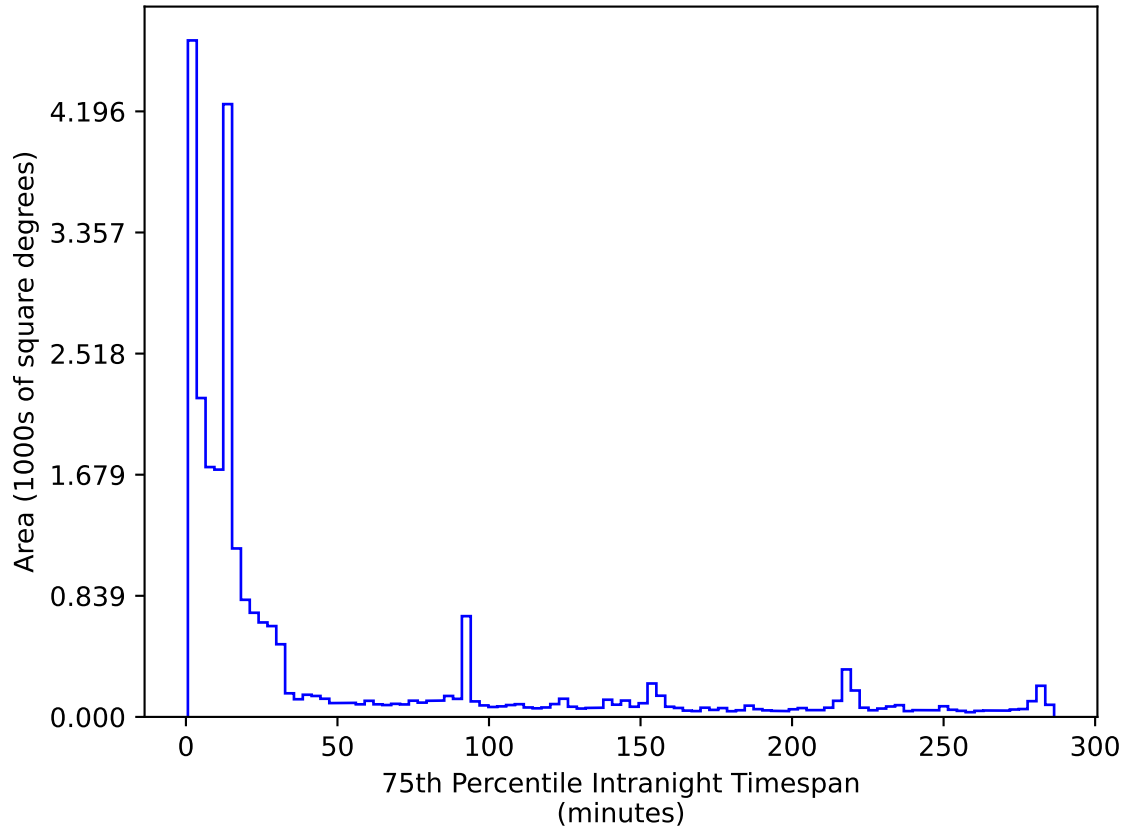
too_ignore_100_1v3.4_10yrs All sky r band: 75th Percentile Intranight Timespan
