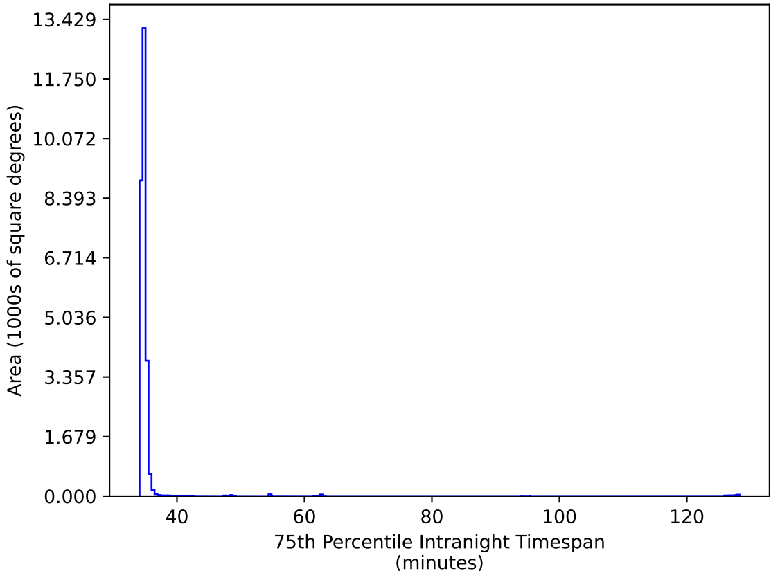
too_ignore_100_1v3.4_10yrs All sky iz bands: 75th Percentile Intranight Timespan
