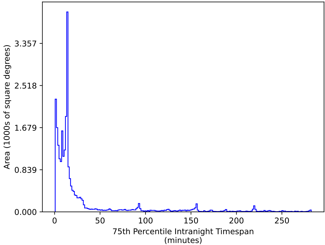
too_ignore_100_1v3.4_10yrs All sky i band: 75th Percentile Intranight Timespan
