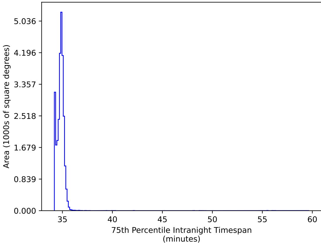
too_ignore_100_1v3.4_10yrs All sky: 75th Percentile Intranight Timespan
