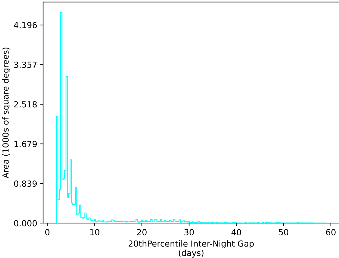
too_ignore_100_1v3.4_10yrs All sky u band: 20thPercentile Inter-Night Gap
