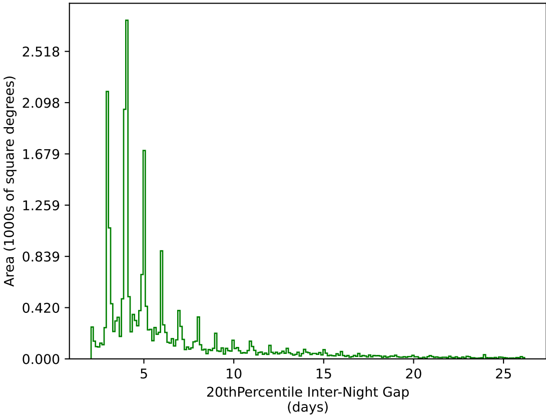
too_ignore_100_1v3.4_10yrs All sky g band: 20thPercentile Inter-Night Gap
