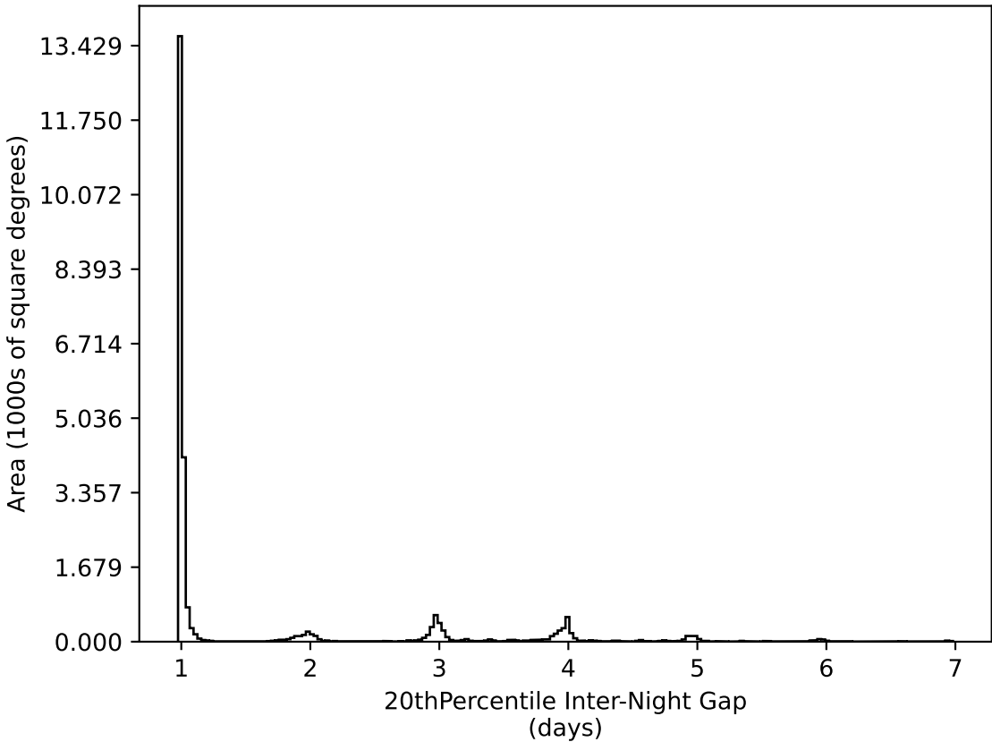
too_ignore_100_1v3.4_10yrs All sky all bands: 20thPercentile Inter-Night Gap
