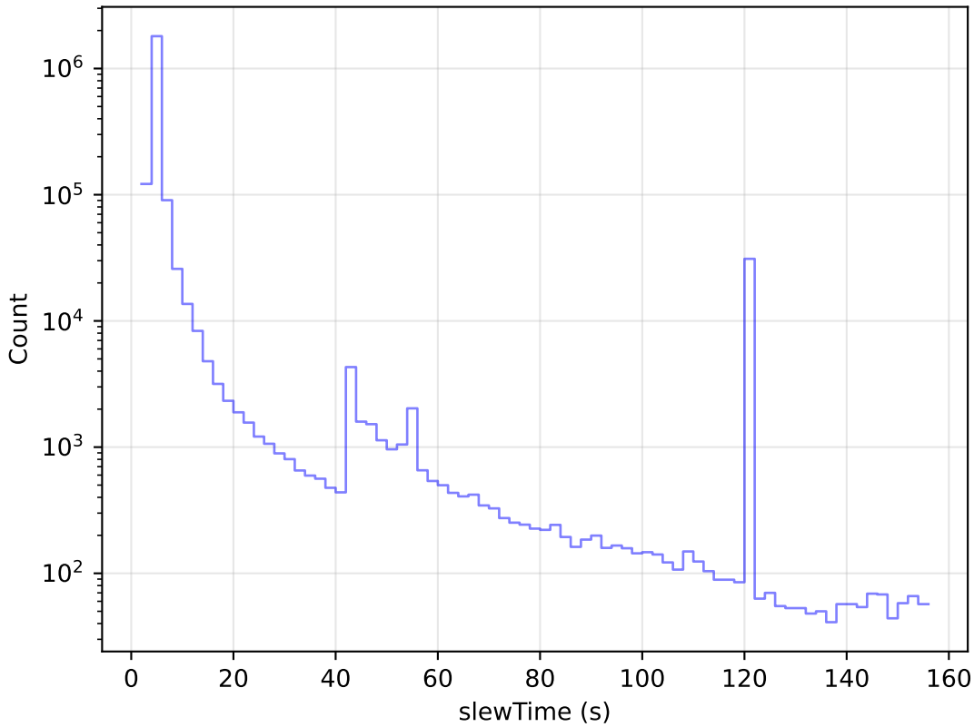
too_ignore_100_1v3.4_10yrs All visits: Slew Time Histogram
