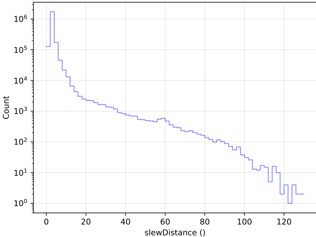
too_ignore_100_1v3.4_10yrs All visits: Slew Distance Histogram
