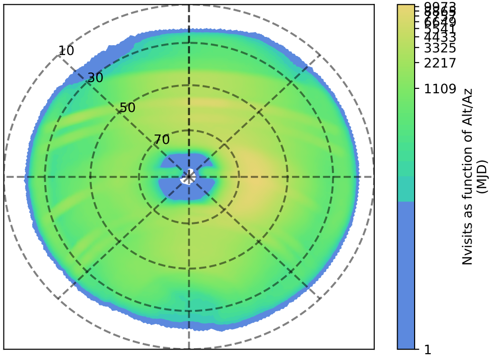
too_ignore_100_1v3.4_10yrs : Nvisits as function of Alt/Az
