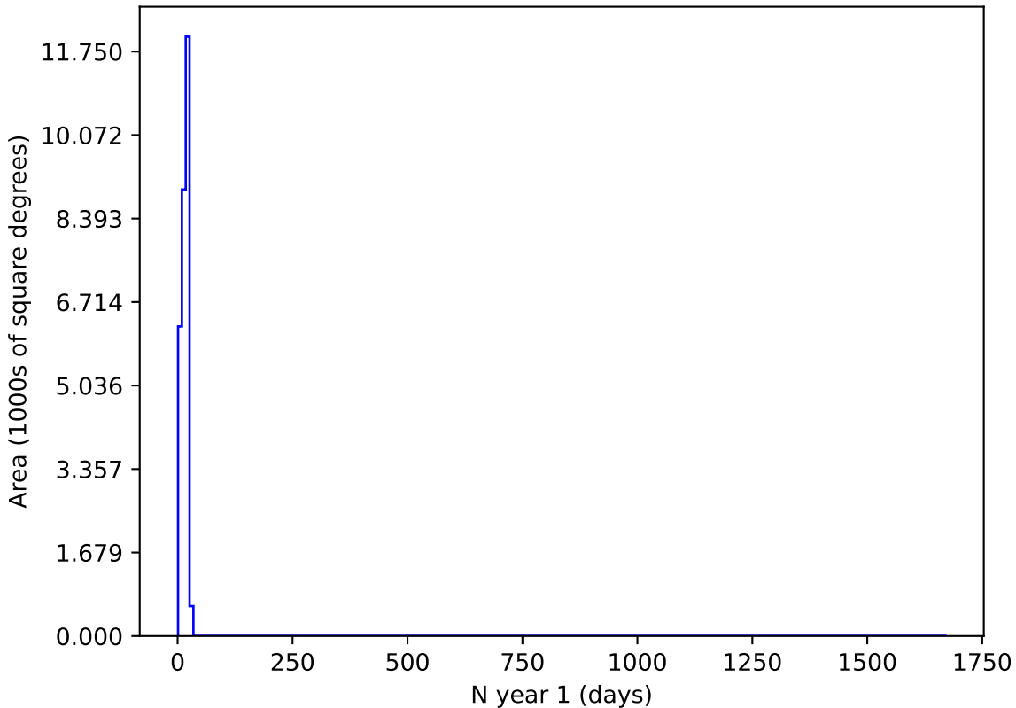
too_ignore_100_1v3.4_10yrs r and night < 365: N year 1
