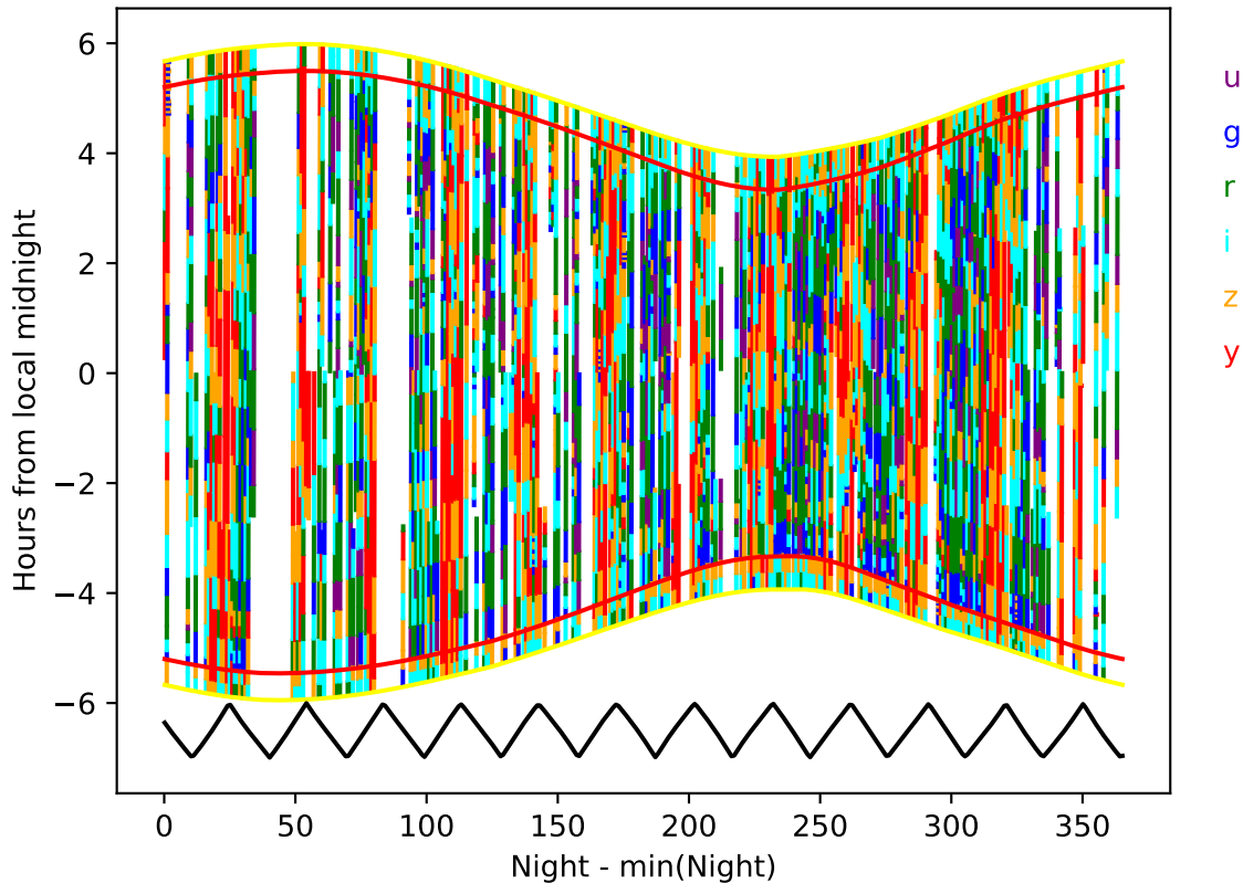
too_ignore_100_1v3.4_10yrs year 4-5: Hourglass
