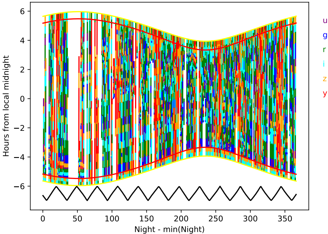
too_ignore_100_1v3.4_10yrs year 2-3: Hourglass
