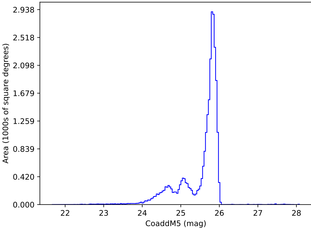
too_ignore_100_1v3.4_10yrs z: CoaddM5
