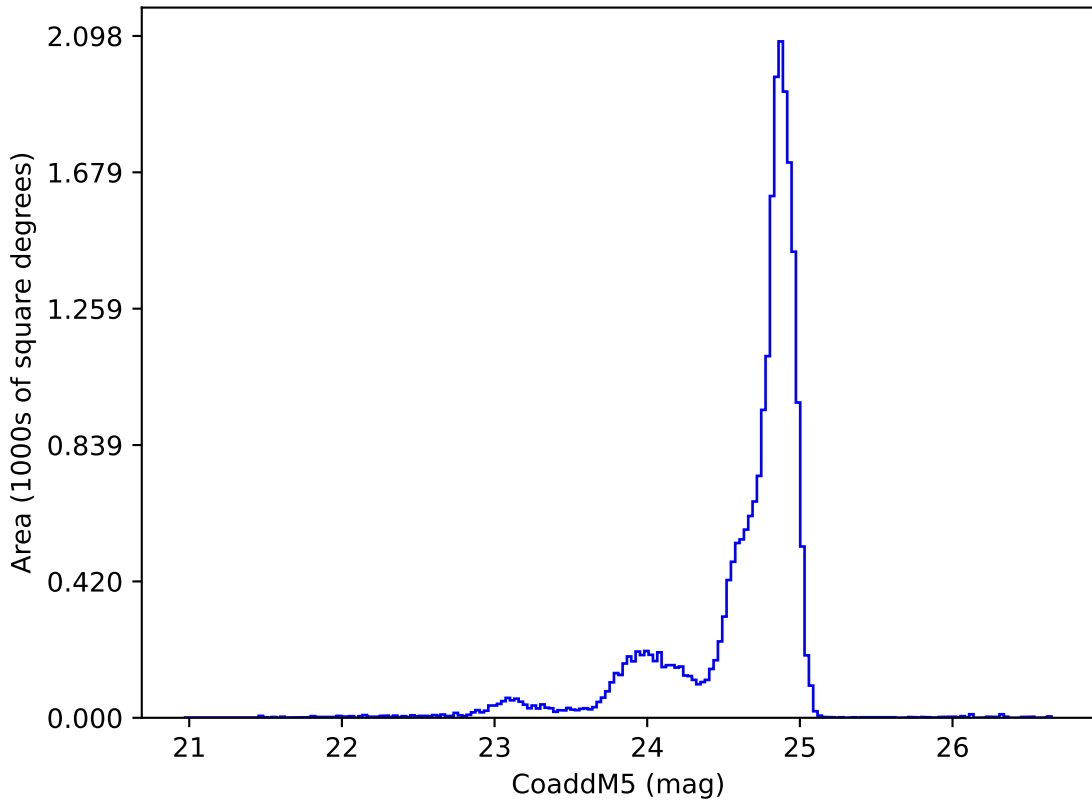
too_ignore_100_1v3.4_10yrs y: CoaddM5
