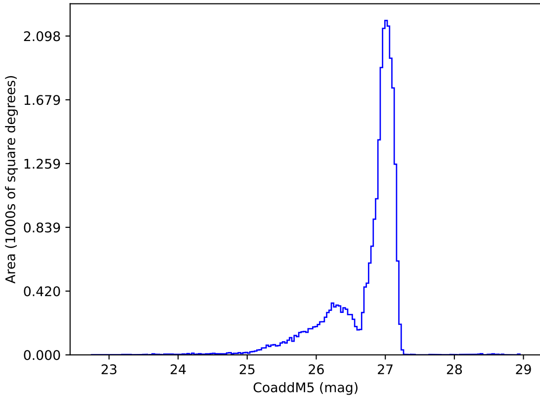
too_ignore_100_1v3.4_10yrs r: CoaddM5
