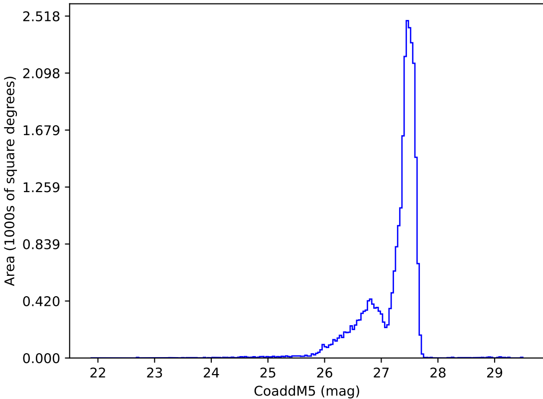
too_ignore_100_1v3.4_10yrs : CoaddM5
