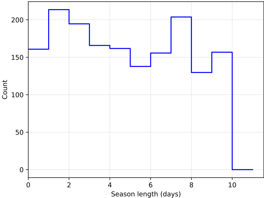
too_ignore_100_1v3.4_10yrs DD:WFD all bands: SeasonLength
