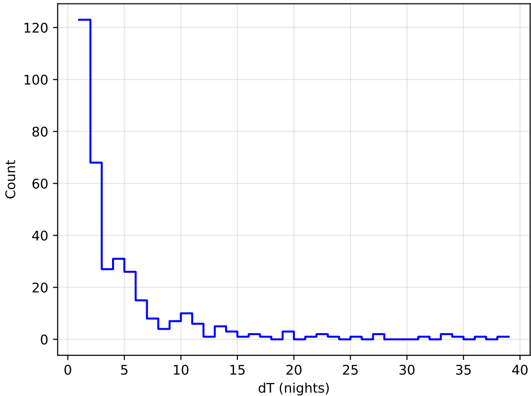
too_ignore_100_1v3.4_10yrs all bands: DD:WFD Delta Nights Histogram
