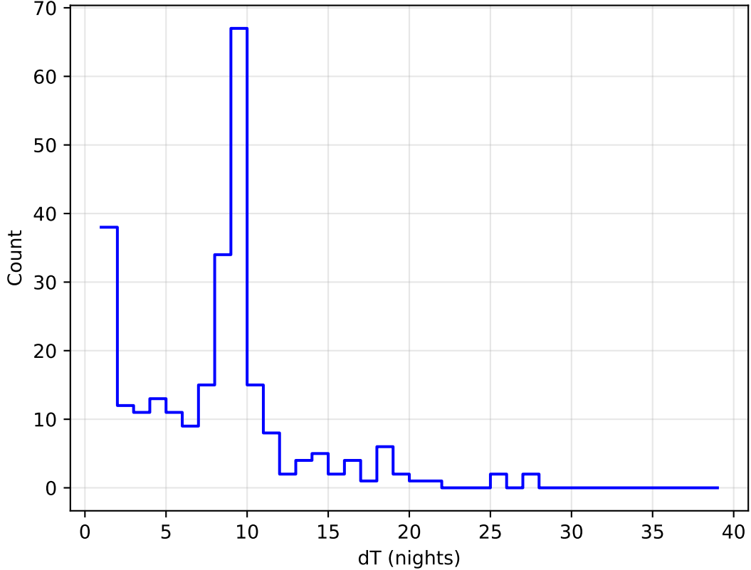
too_ignore_100_1v3.4_10yrs all bands: DD:ELAISS1 Delta Nights Histogram
