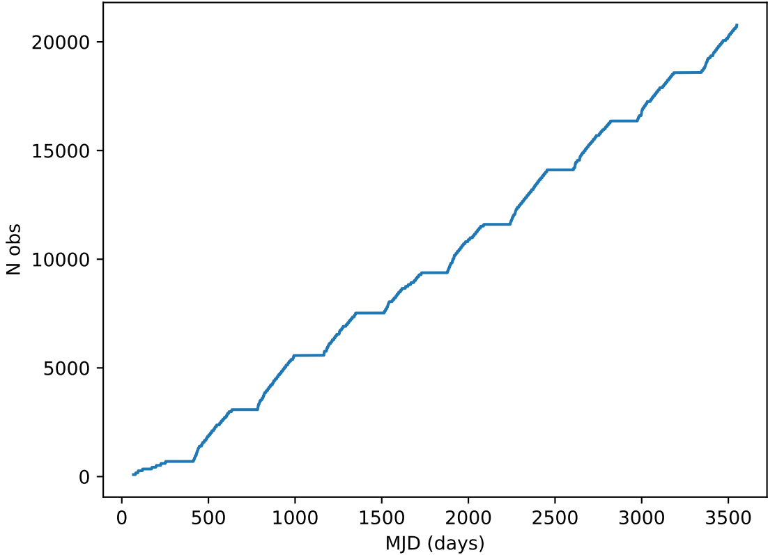
too_ignore_100_1v3.4_10yrs all bands: DD:ELAISS1 Cumulative NVisits
