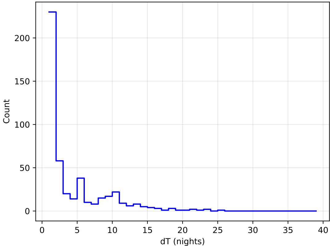
too_ignore_100_1v3.4_10yrs all bands: DD: COSMOS Delta Nights Histogram
