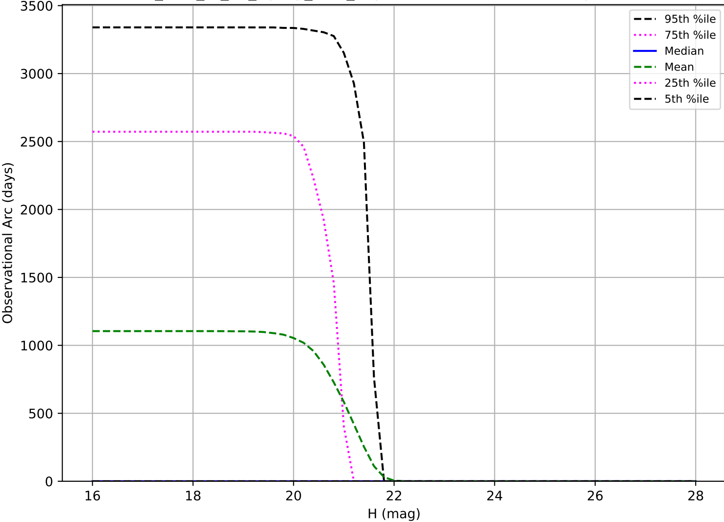
too_elab_r8_d3_ugrizy_v3.4_10yrs: Observational Arc Length Vatira
