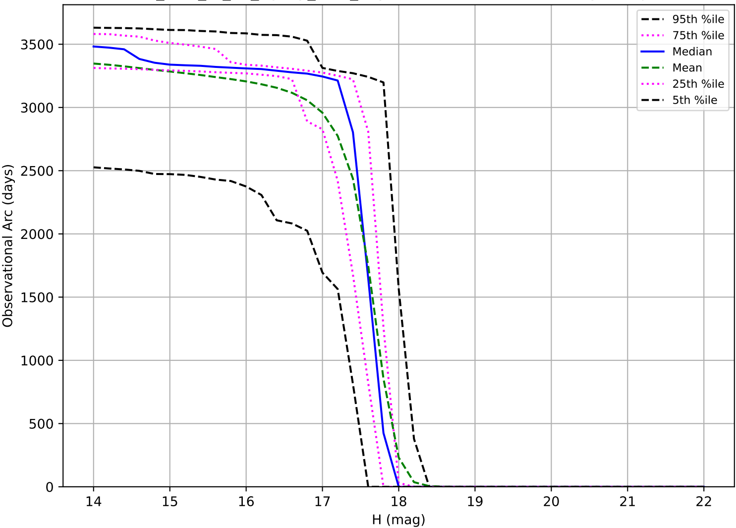
too_elab_r8_d3_ugrizy_v3.4_10yrs: Observational Arc Length Trojan
