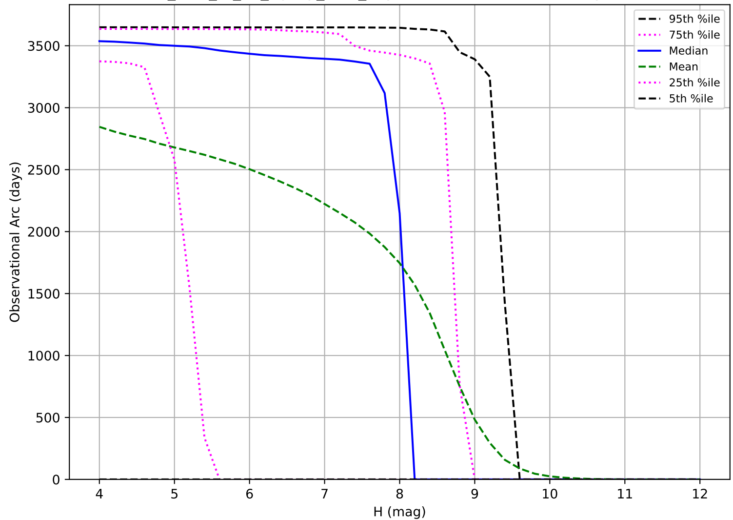
too_elab_r8_d3_ugrizy_v3.4_10yrs: Observational Arc Length TNO
