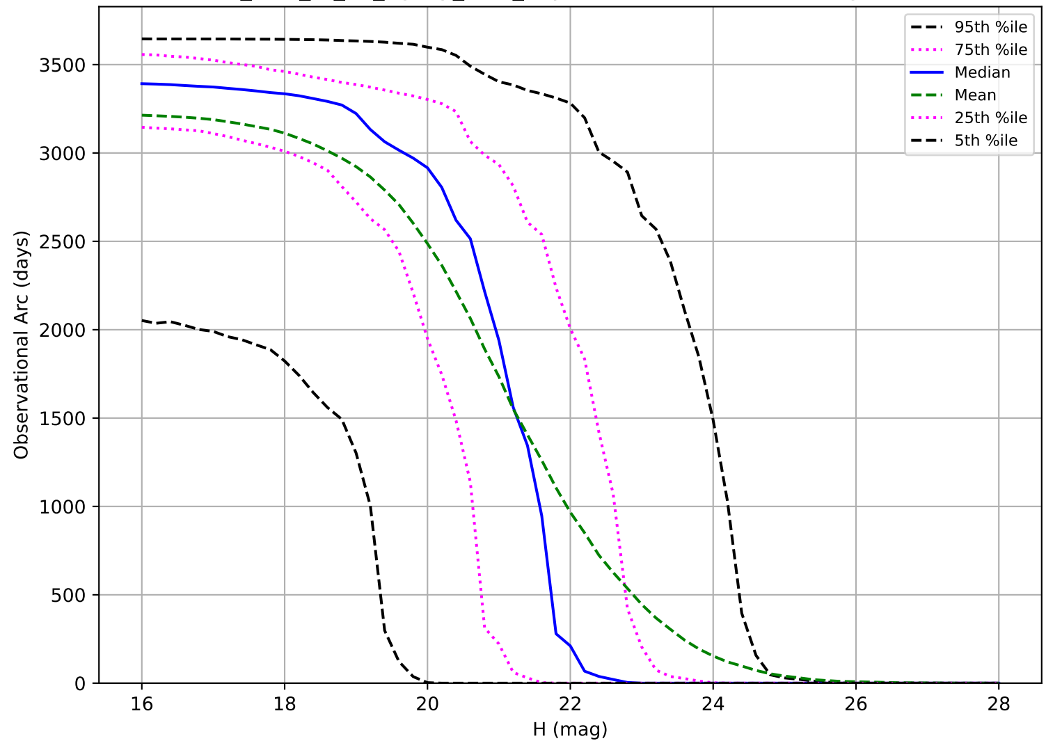
too_elab_r8_d3_ugrizy_v3.4_10yrs: Observational Arc Length PHA
