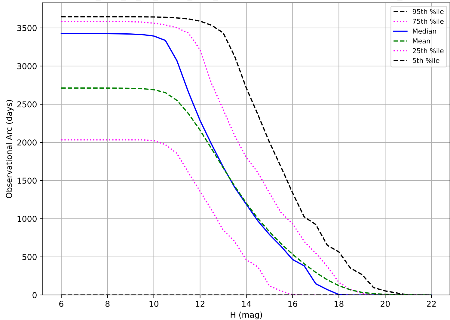
too_elab_r8_d3_ugrizy_v3.4_10yrs: Observational Arc Length OCC_r5
