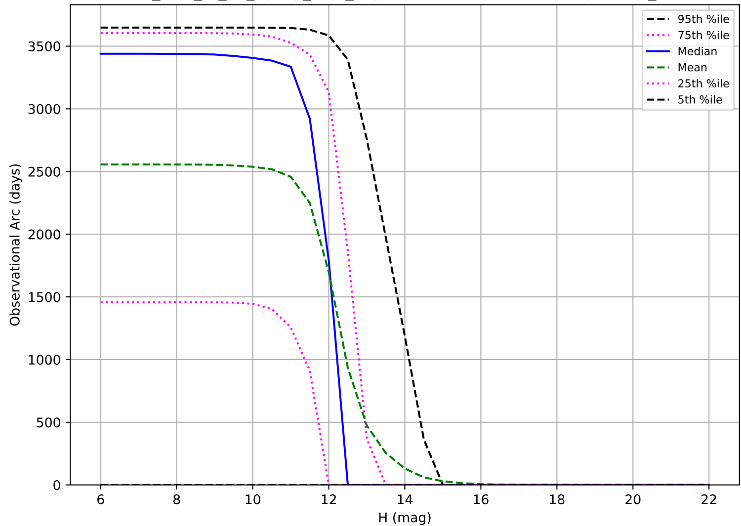
too_elab_r8_d3_ugrizy_v3.4_10yrs: Observational Arc Length OCC_r20
