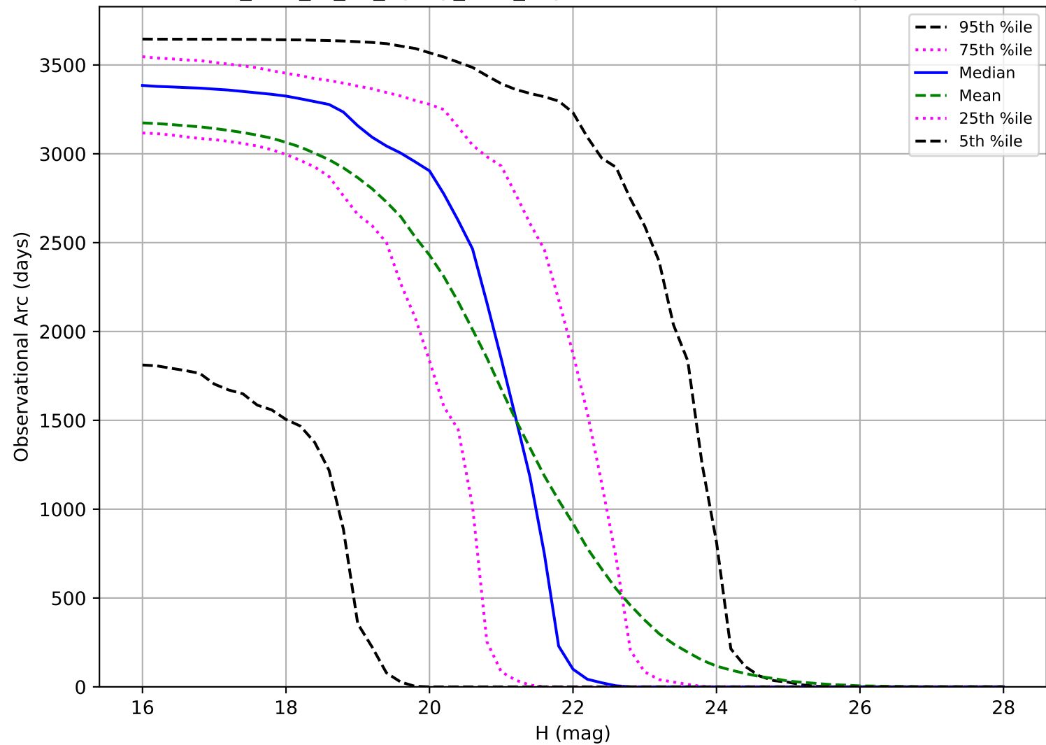
too_elab_r8_d3_ugrizy_v3.4_10yrs: Observational Arc Length NEO
